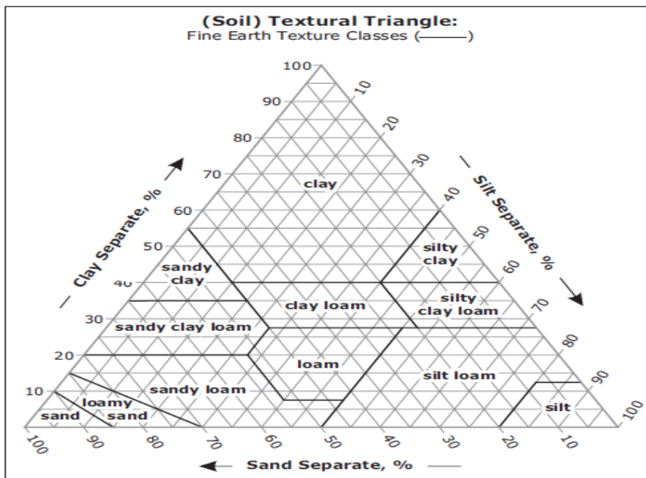
Figure 7: Triangular Diagram of Soil Textural Classes (USDA Triangle).
