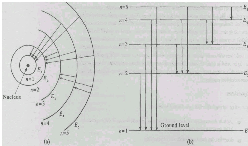
Fig. 2.1 (a) Bohr circular orbits for the revolving electron of hydrogen atom, showing transitions, giving rise to the emitted light waves of different frequencies; (b) Energy level diagram for the hydrogen atom
