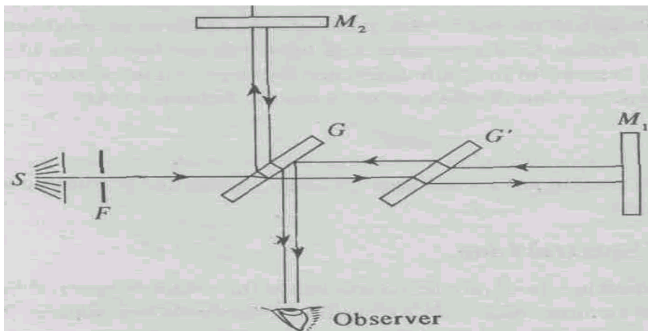
Fig. 1.3 Light paths for Michelson Interferometer
