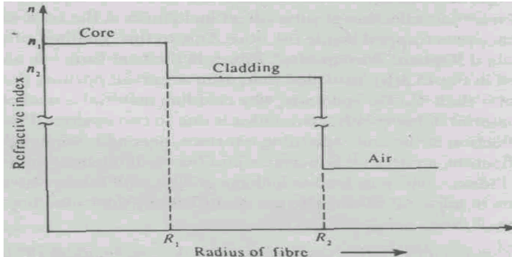
Fig. 4.4: Refractive index profile of a step-index fibre
