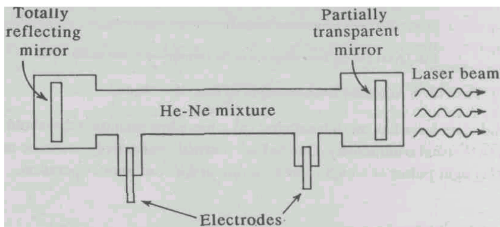
Fig. 2.12 The He-Ne Laser
