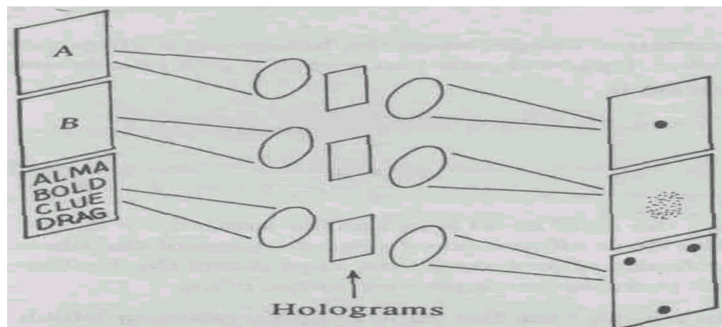
Fig. 3.8 Pattern recognition by holographic vander Lugt filter. (The holograms are seen between the lenses.)
