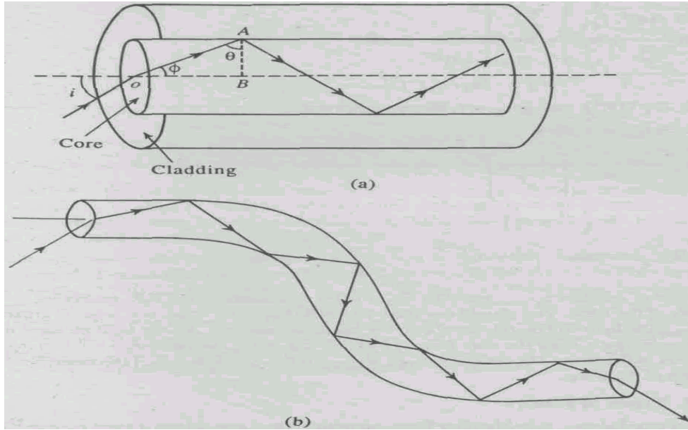
Fig. 4.3: (a) Light propagation through a fibre by total internal reflection. (b) Light propagation through a bent fibre
