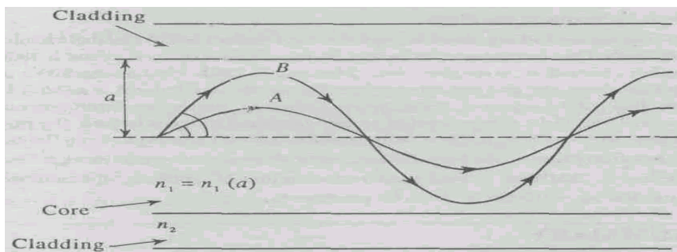
Fig. 4.10 Two rays A and B travelling through a GRIN-fibre
