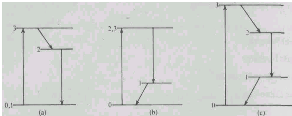
Fig. 2.8: Three level pumping schemes, (a) the ground state (0) and lower lasing state (1) are the same, (b) pumping state (3) and upper lasing state (2) are the same, (c) Four level pumping scheme
