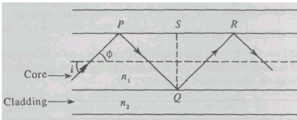
Fig. 4.9 Ray of light passing through a step-index fibre
