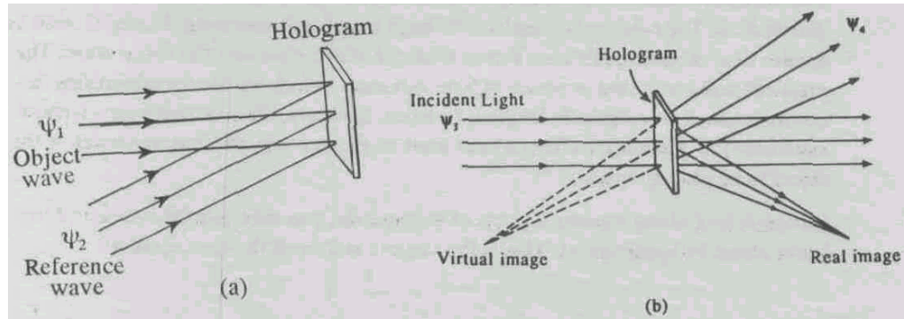
Fig. 3.5: (a) Recording the hologram: Wave reflected from an object interferes with the reference wave, (b) Reconstruction: The hologram diffracts the reconstruction wave, resulting in transmitted wave which produces a real and a virtual image
