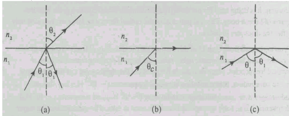
Fig. 4.2 Total Internal reflection
