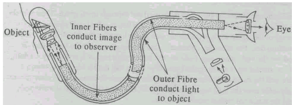
Fig. 4.6 Flexible fibrescope
