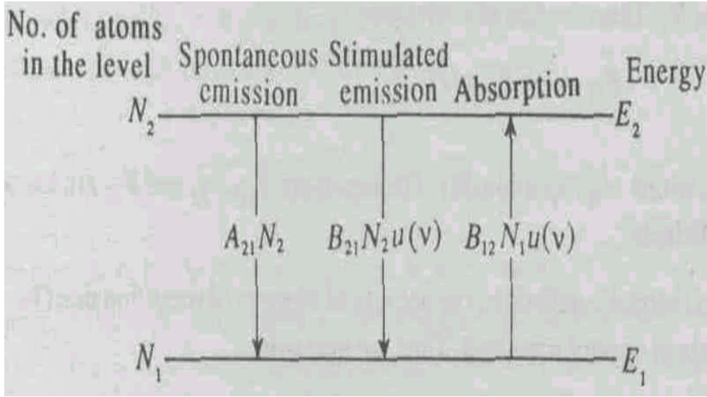
Fig. 2.3 An atomic system of two energy levels showing different emission and absorption processes
