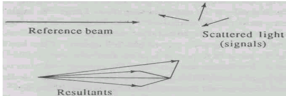
Fig. 3.2 Addition of a strong coherent reference beam (top left) with random-phase signals (top right) gives similar resultant (bottom)
