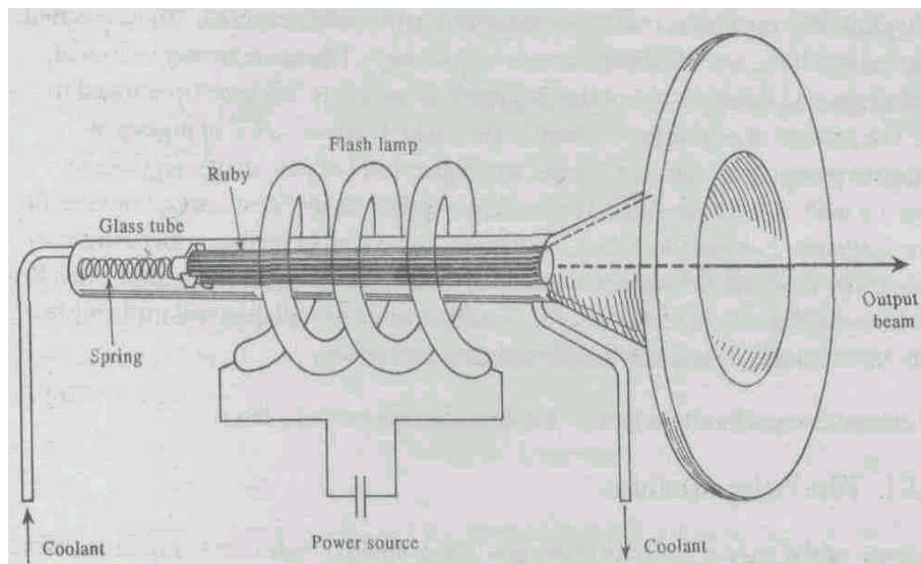
Fig. 2.5 The Ruby laser
