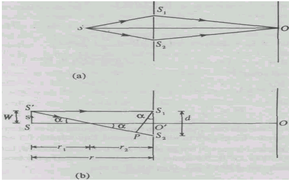
Fig. 1.4 (a) Young's double slit experiment with a point source, S, (b) Young's double slit experiment with an extended source S' S
