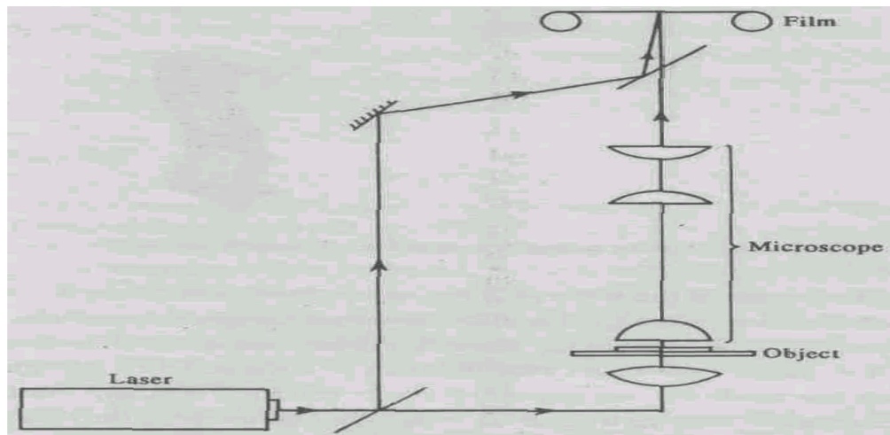
Fig. 3.6 Holographic microscope
