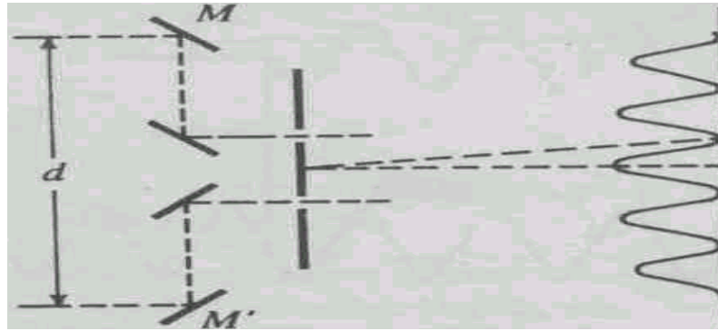
Fig. 1.5 Michelson's stellar interferometer
