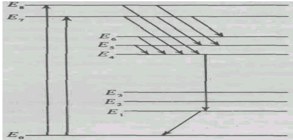
Fig. 2.11: Energy level diagram of Nd (neodymium) ion in Nd: YAG
