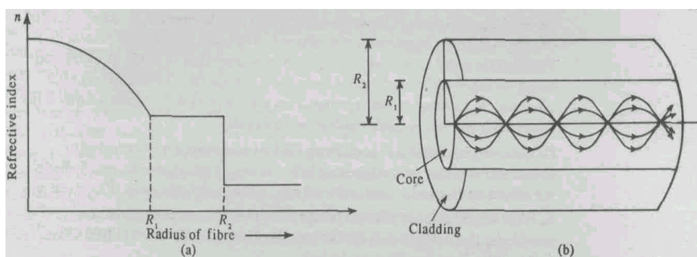
Fig. 4.5 (a) The refractive index profile of a Gradient-Index fibre; (b) Ray paths in such a fibre
