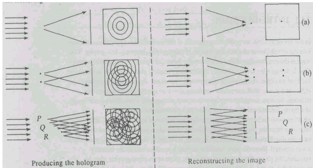
Fig. 3.1 The principle of holography: (a) Point object forming concentric diffraction rings as in zone plate; reconstruction of zone plate gives point image (top right). For two points and a more complex object, these features are shown in (b) and (c) respectively
