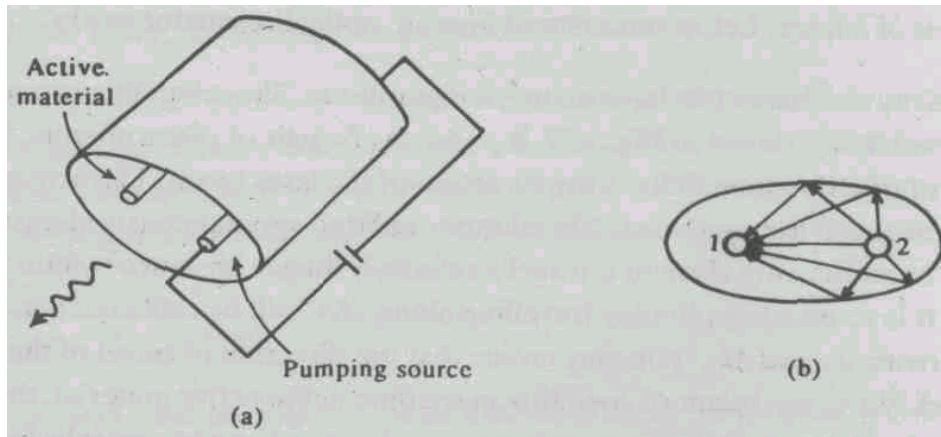
Fig. 2.10: Pumping arrangement for solid-state lasers
