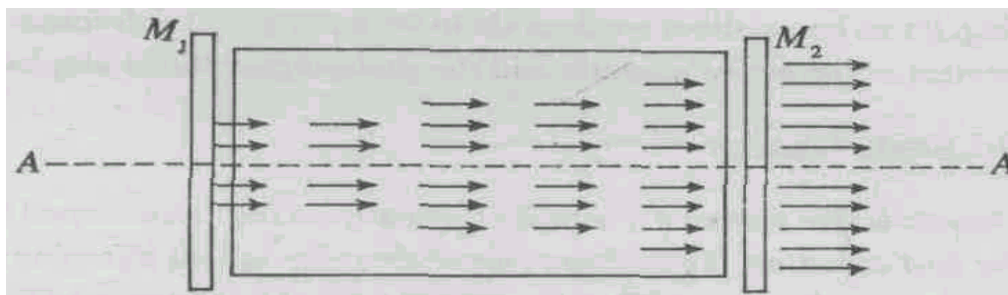
Fig. 2.9: Optical resonator consisting of two mirrors M_1 and M_2 ; M_1 is totally reflecting whereas M_2 is semitransparent; the axis of the mirrors is aligned with that of the active material
