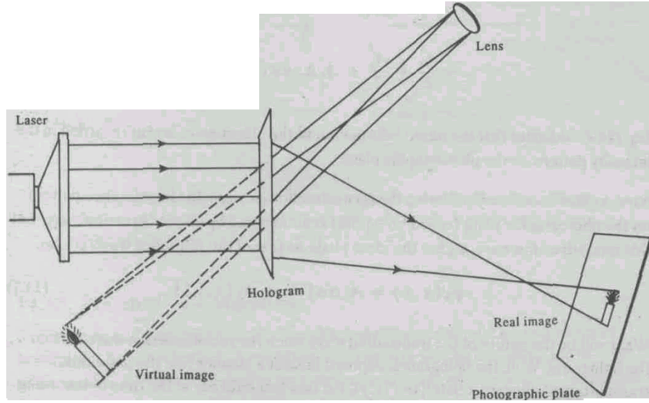
Fig. 3.4 Reconstruction process of an Image in holography
