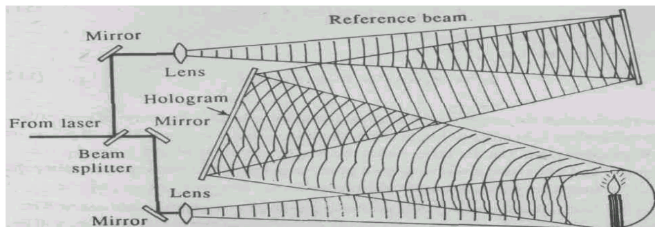
Fig. 3.3: Recording the hologram; microscope lenses broadens both beams without affecting their coherence
