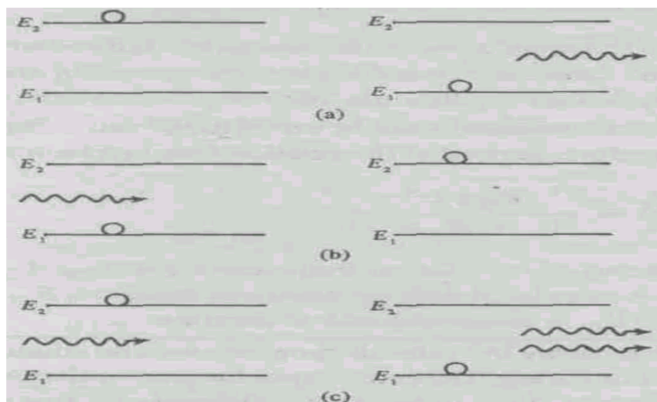
Fig. 2.2 (a) Spontaneous Emission (b) Absorption and (c) Stimulated Emission of light
