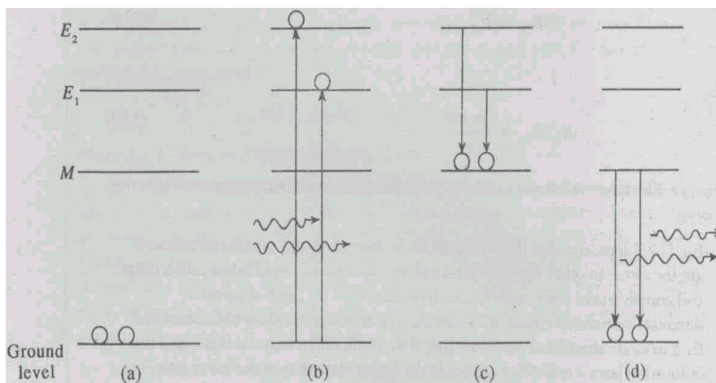
Fig.2.4: Energy levels of chromium atom: (a) atoms in the ground state
