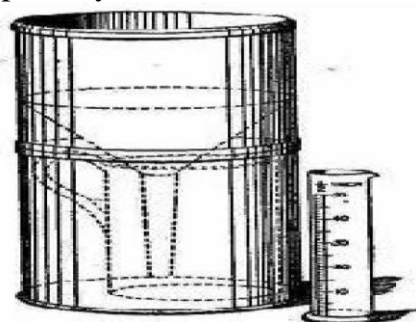
FIG. 1.51.—Standard rain-gauge.
