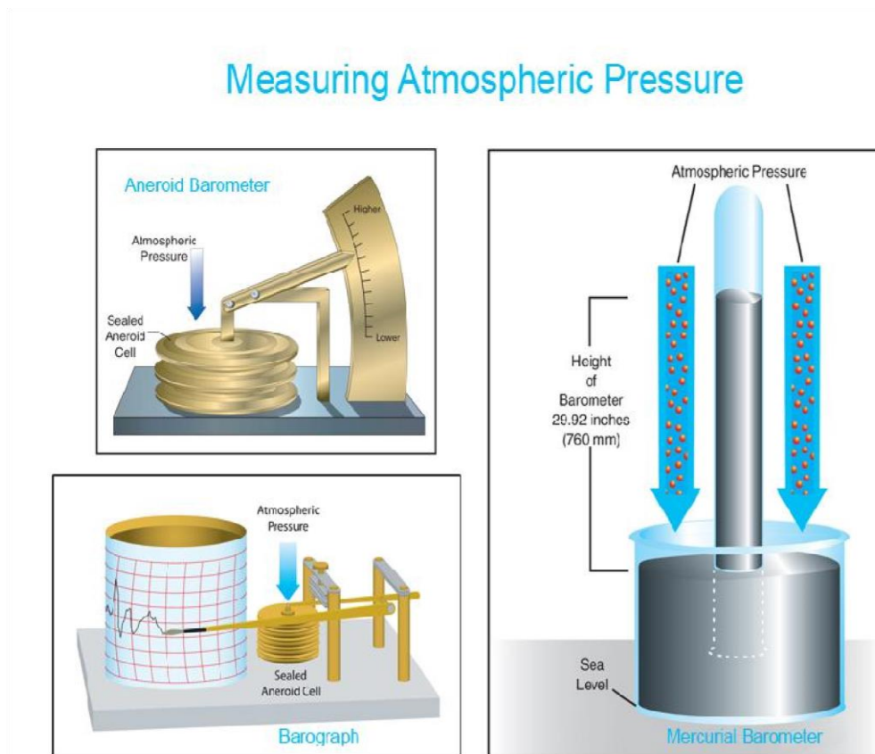
Fig. 1.7: Three Common Instruments (mercurial barometer, aneroid barometer and barograph) for Measuring Atmospheric Pressure
