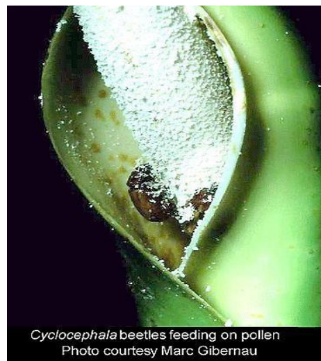
Fig. 9.14: Cyclocephala beetles
