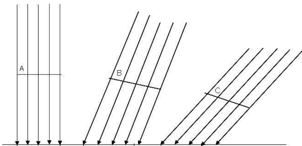
Fig. 2: Sun's Angle
