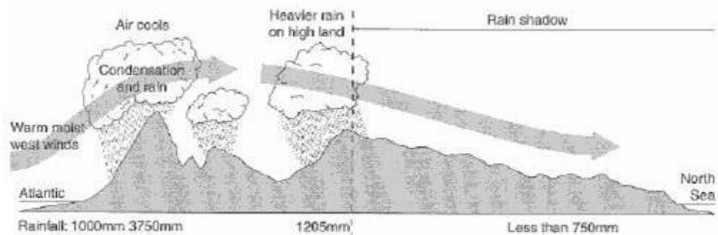
Fig. 7: Relief Rainfall
