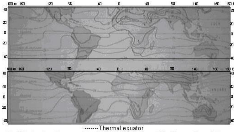
Fig. 10: Sea level temperatures in July and January ( ^{\circ}\text{C} ). The position of the thermal equator (temperatures reduced to sea level)
