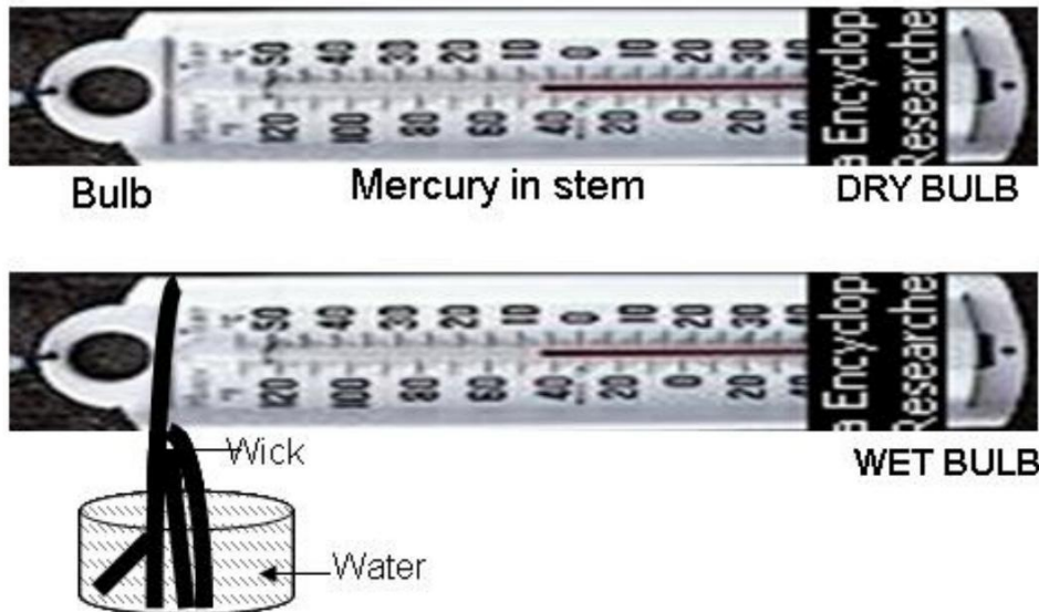
Fig. 16: Hygrometer (Dry and Wet bulb thermometer)
