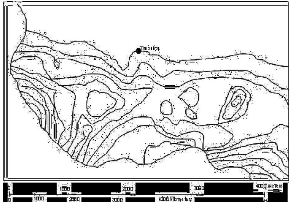
Fig. 12: August rainfall over West Africa (inches)
