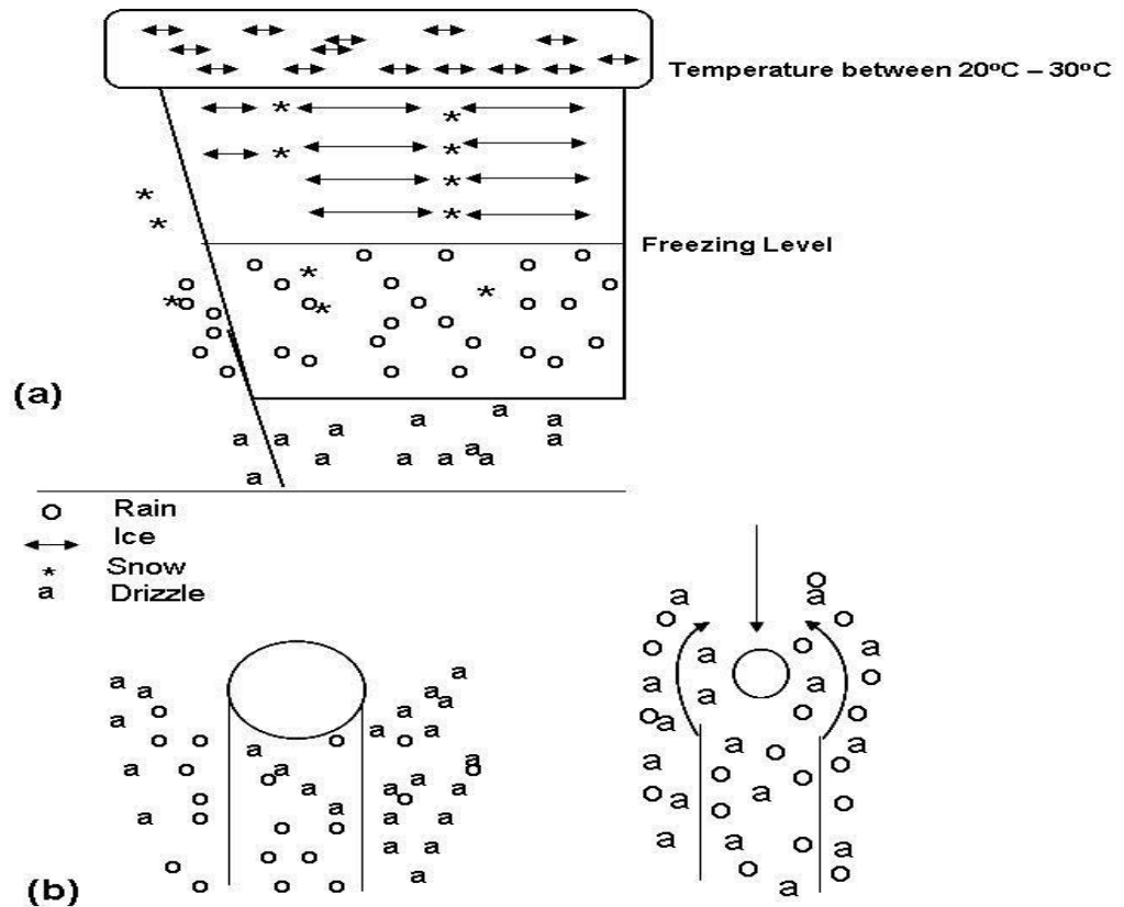
Fig. 5: Processes of raindrop formation according to (a) Bergeron-Feideisen theory and (b) coalescence theory (Source: Ayode, 2004)
