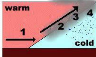
Fig. 8: Frontal rainfall
